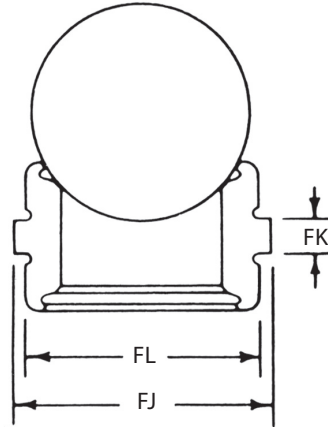
RIB SEAT
